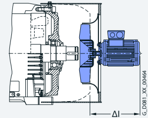
Frame sizes 225 to 315
