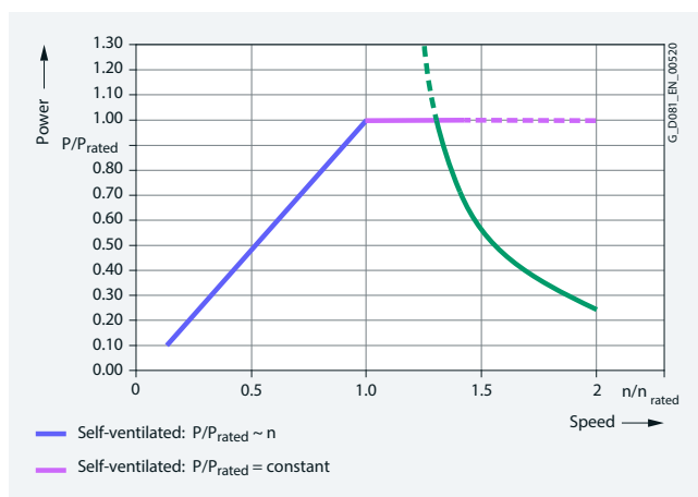
Power limit for Innomotics GP/SD VSD4000 line self-ventilated
