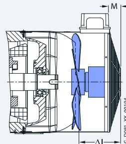
Frame sizes 100 to 200
