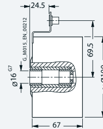
Mounting dimensions of LL 861 900 220 rotary pulse encoder
