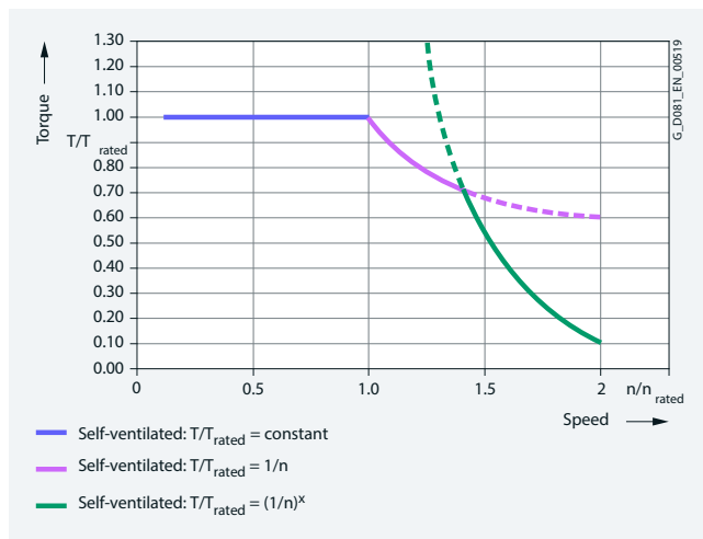
Torque limit for Innomotics GP/SD VSD4000 line self-ventilated
