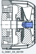
Fig. 9 Prepared for mountings, center hole only (for BFK458 brake, order code F01 and/or encoder order code G04/G05/G06/G11/G12 , order code G40 (up to frame size 160, standard with frame size 180 and above)
